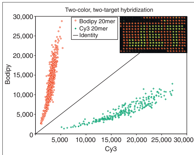
Figure 9 Sensitivity to mismatches as demonstrated by two-color hybridization. An array was synthesized containing reporters complementary to targets 5'-Cy3-GAC CTC CCG CTC ACG CAC CT (green) and 5'-Bodipy-GAC CTC CCG GAC ACG CAC CT (red), using standard conditions described in Materials and methods. The bases in bold are different in the two reporter:target molecules. The slide was hybridized with an equimolar mixture of the two labeled target oligonucleotides and the fluorescence intensity determined on the ScanArray 5000 using the Dapple spot-finding program. The green/red ratios of the green- and red-complementary features were 3.12 \pm 0.57 ( N = 230 ) and 0.25 \pm 0.05 ( N = 660 ), respectively. Graphing Cy3 intensity vs Bodipy intensity shows excellent separation between signals and the insert shows that the effects of two base changes are clearly distinguishable by eye.
