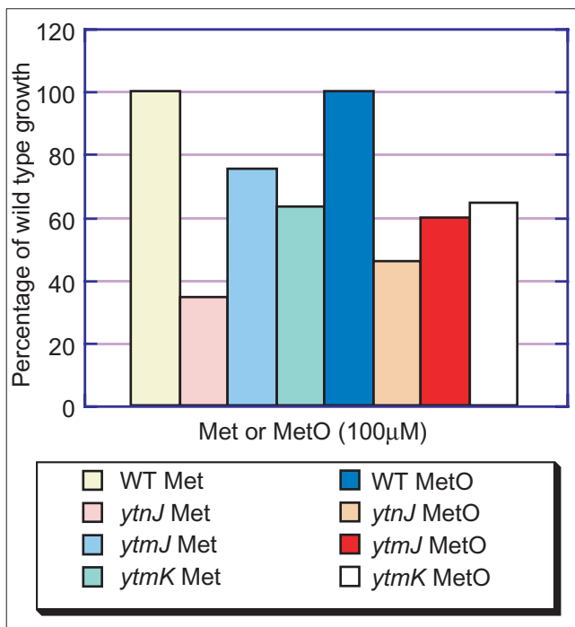
Figure 2 Comparison of the growth of B. subtilis wild type (WT) with ytnJ , ymJ and ymK mutants (BFS70, BFS85 and BFS86, respectively) on methionine (Met) and methionine sulfoxide (MetO) at 100 μM concentration. Growth was measured after 7 h and is represented as a percentage of wild-type growth.
