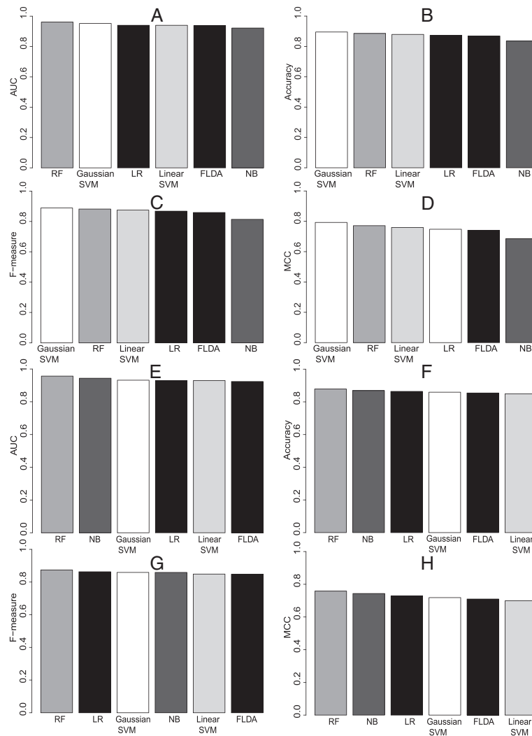
Figure 3 Evaluation of site-level mirMark. Performance of site-level mirMark using various classification methods according to (A) AUC, (B) accuracy, (C) F-measure, and (D) MCC using 10-fold cross-validation. Similarly, the performance is shown using a hold-out test set (E-H).
