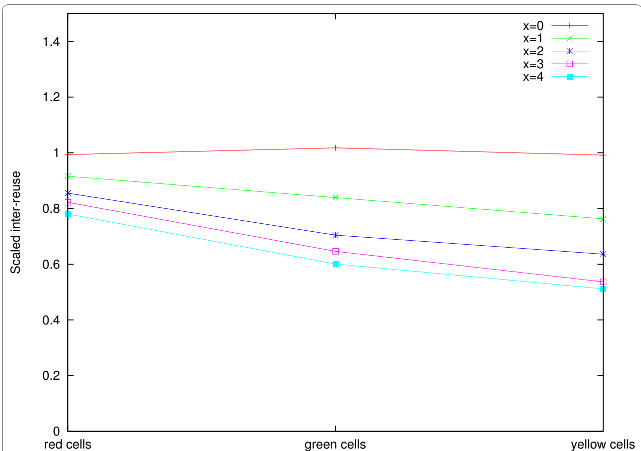
Figure 10 The scaled inter-reuse for five simulated genomes M, R, D, Q, H on m = 2,000 synteny blocks, n = 900 fragile regions, and the turnover rate x varying from zero to four with the phylogenetic tree and branch lengths shown in Figure 4. The simulations follow FBM ( x = 0 ) and TFBM ( x varies from one to four). The plot shows the scaled inter-reuse for only three reference points (corresponding to red, green, and yellow cells) that are somewhat arbitrarily connected by straight segments for better visualization.
