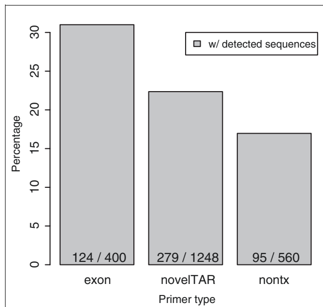
Figure 1 Frequency of PCR products obtained from different genomic regions. Primers designed to the sense and antisense strands of exons, novel transcriptionally active regions (TARs) and nontranscribed regions were used to generate rapid amplification of cDNA ends (RACE) products. The frequency of PCR products obtained is indicated. nontx, region not previously shown to be transcribed.
