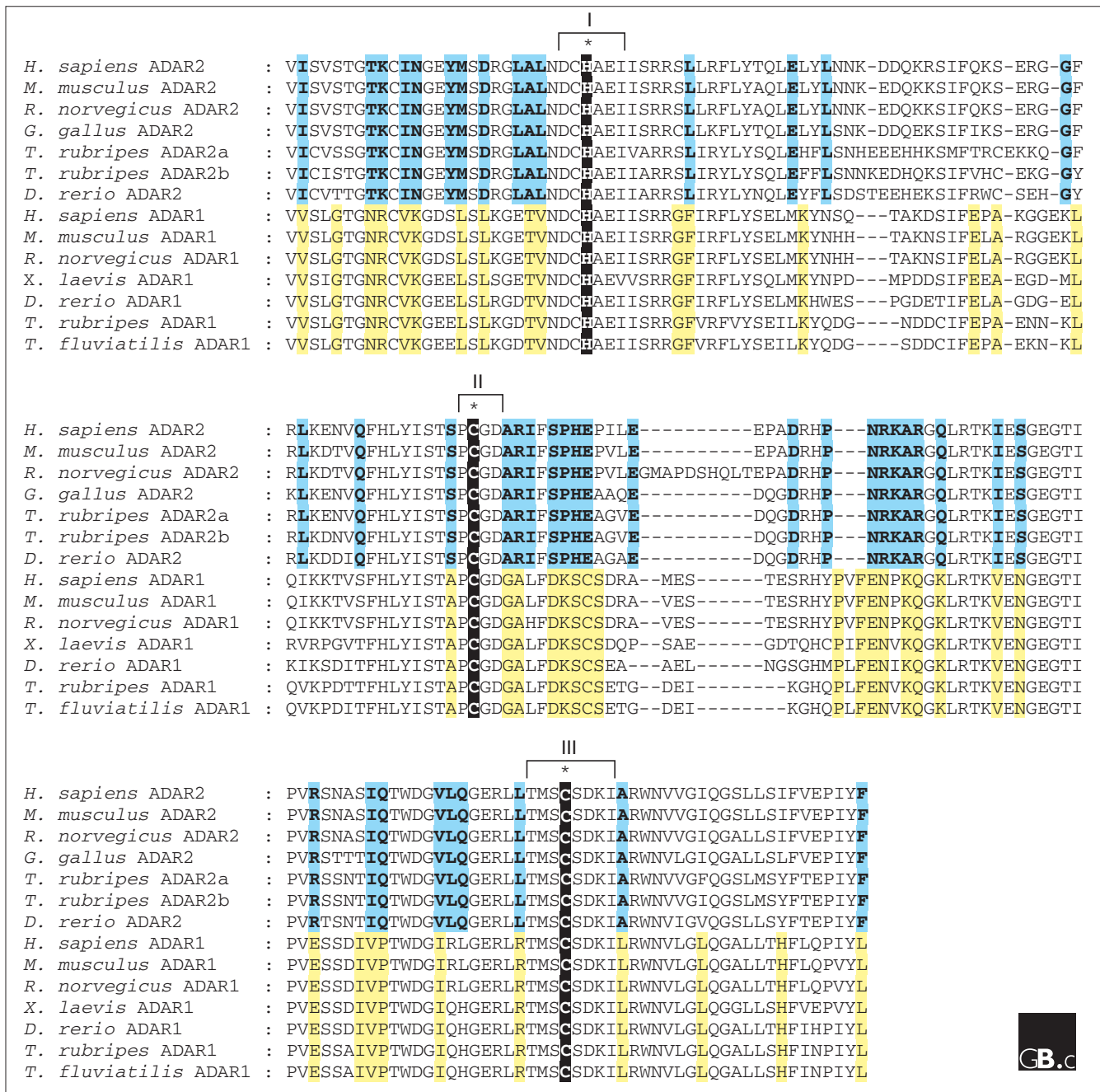
Figure 3 An alignment of core deaminase domains from vertebrate ADAR1 and ADAR2 proteins, showing residues characteristic for each. Asterisks indicate cysteines and histidines that chelate zinc, as in Figure 1, and the three active-site motifs are bracketed.
