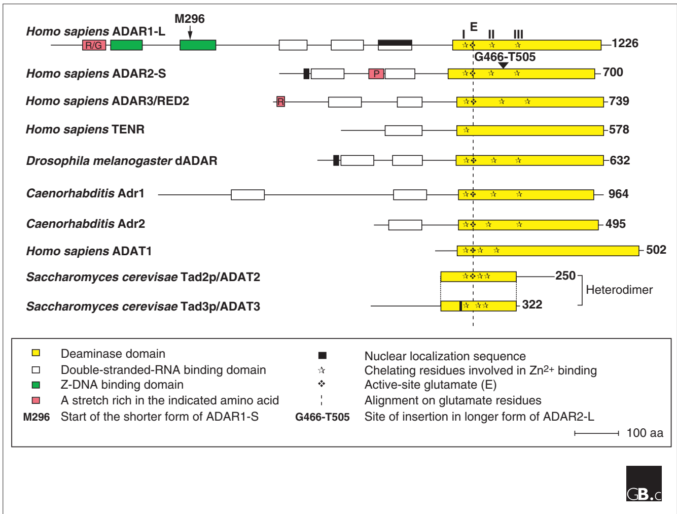
Figure 1 Primary structures of ADARs and ADATs (adenosine deaminases acting on tRNAs), showing arrangements of dsRNA-binding domains and deaminase domains. The deaminase motifs (I-III) consist of four or five highly conserved amino acids surrounding each of the cytosines and histidines that bind zinc. Proteins have been drawn to scale and are aligned at the catalytic glutamate residue (E) in the active site in adenosine deaminase motif I. The deaminase domains of ADAR and ADAT1 proteins are larger than the core deaminase domain (which we define as the region of homology between Tad2/ADAT2 and Tad3/ADAT3) because of the insertion of sequence between the second and third zinc-chelating residues, separating deaminase motifs II and III, and probably also because of fusion with a carboxy-terminal subdomain of unknown origin. Abbreviation: aa, amino acids.
